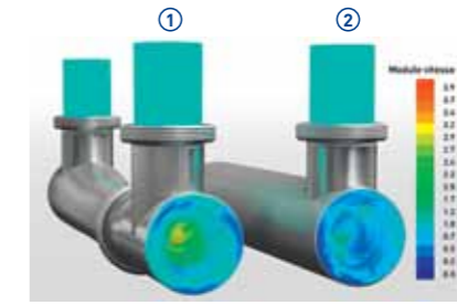
Effect of the inlet tangential design on the speed of the CIP fluid at the rear of the pump. ① HyCare™ design with tangential inlet connection ② Classic design
