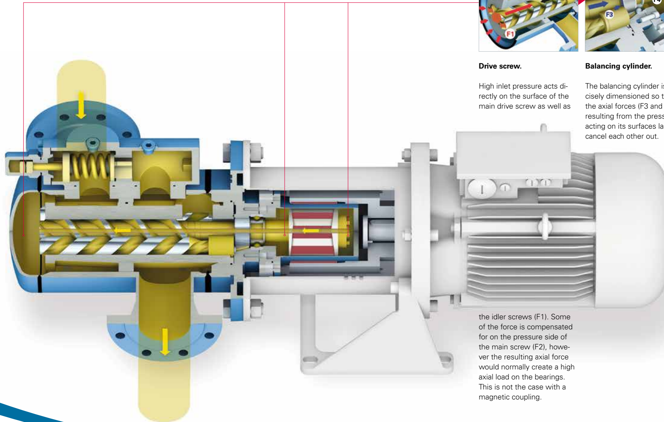
Magnetic coupling.
